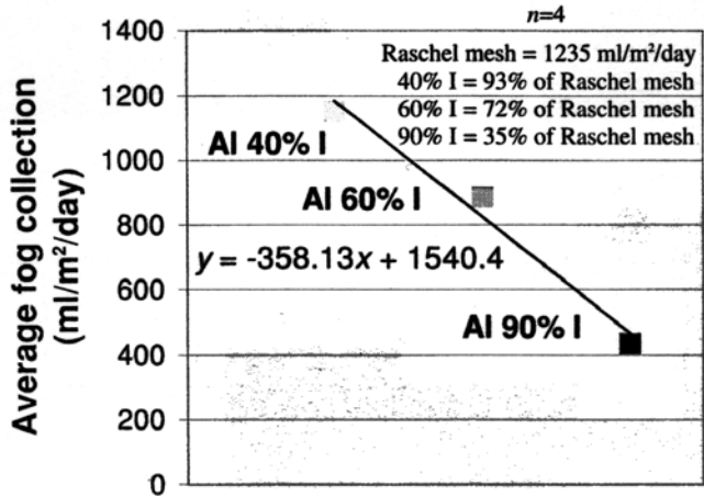
Aluminet fog collector (% shade coefficient)
